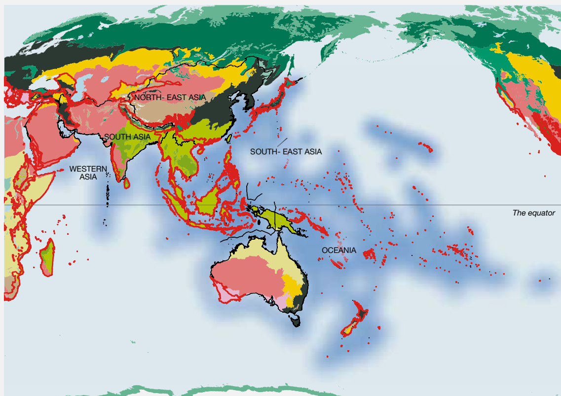
Figure SPM 1 Major ecoregions and the five geographical subregions of the Asia-Pacific region as defined by IPBES.
